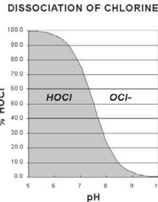
Figure 1 - Equilibrium of Free Chlorine
