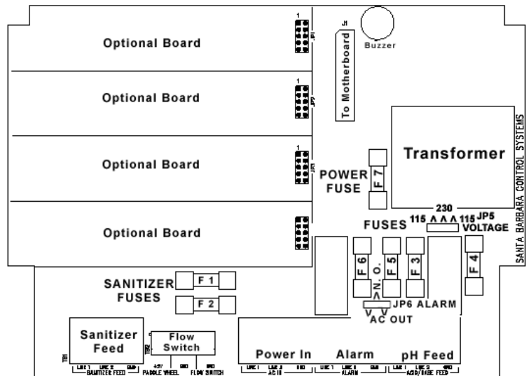
Figure 9 – Power Board
