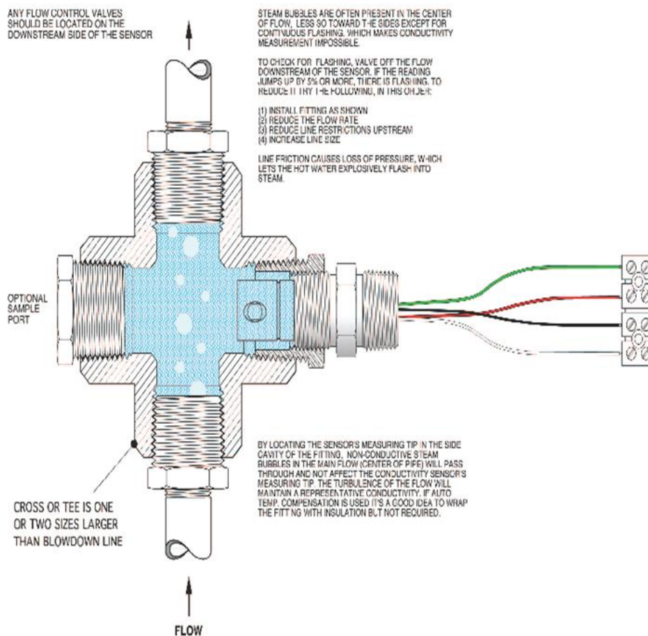
Figure 1. Sensor Orientation
