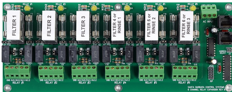
Figure 23. Backwash Relay Expander
