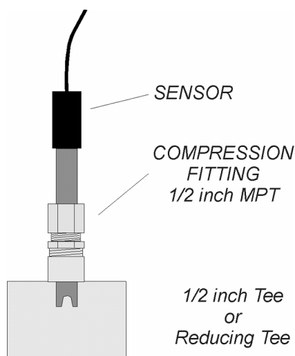
Figure 29. Sensor Installation
