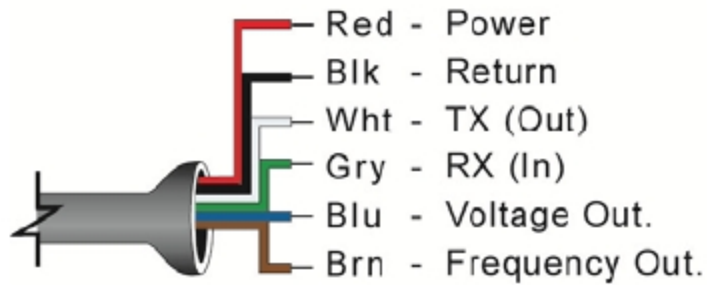
Figure 48. DL-10 Wiring
