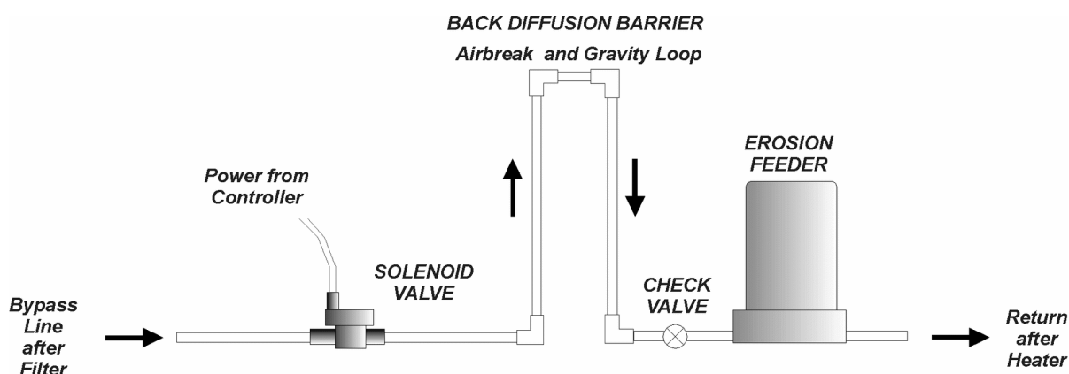
Figure 54. Erosion Feeder Control
