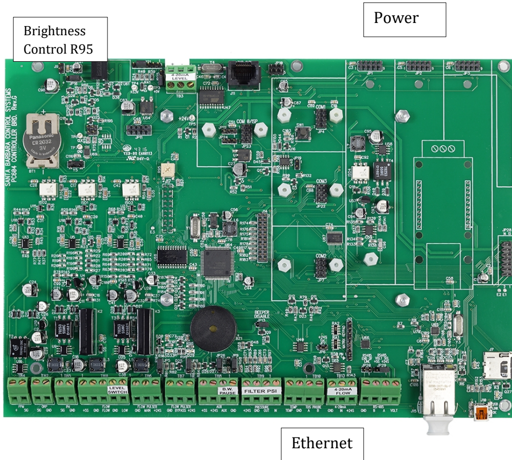
Figure 11. PC 604 CPU Board
