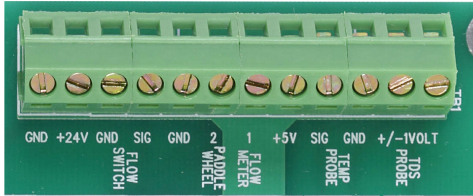
Figure 44. Connections to PC2100 (Power supply board)
