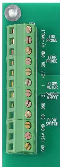
Figure 18. Sensor Connections on Power Board
