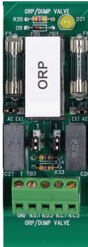
Figure 17. Typical Relay
