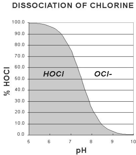
Figure 2 Equilibrium of Free Chlorine.
