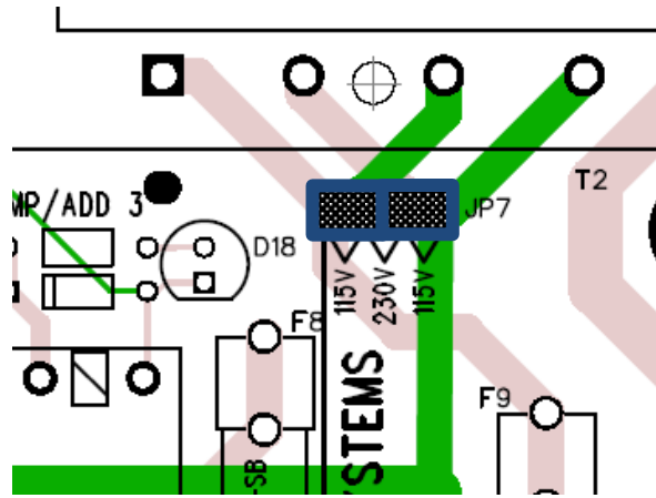
Figure 15. Voltage Selector Jumpers set to 115 volts (2 jumpers)
