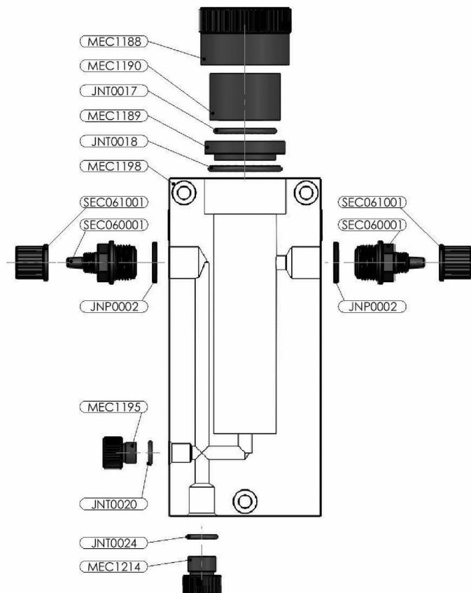
Figure 33. PPM Sensor and Mount
