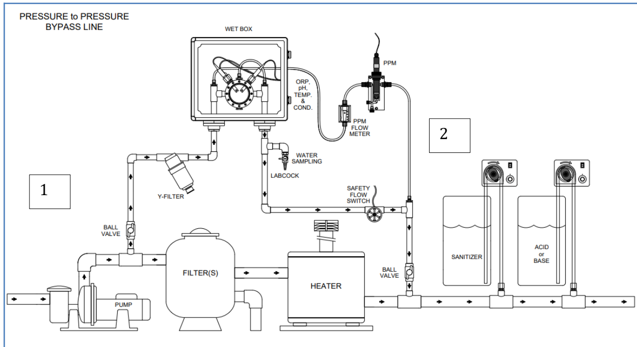
Figure 8. Pressure to Pressure Bypass Line
