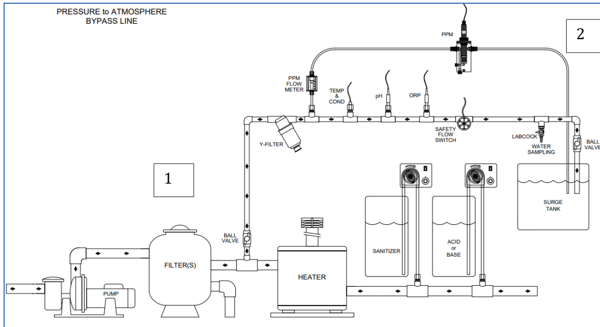
Figure 7. Pressure to Atmosphere Bypass Line
