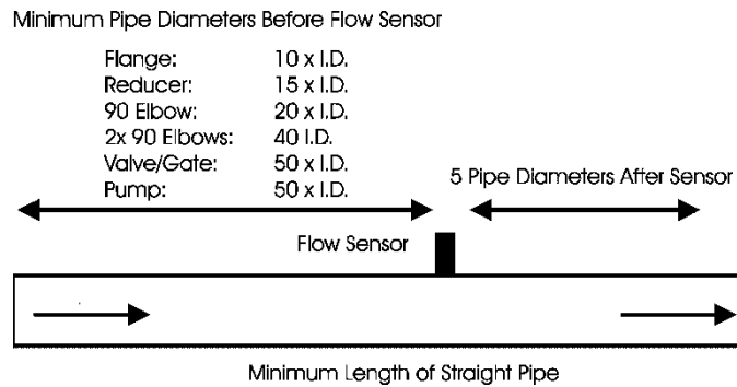
Figure 43. Flow Sensor Location
