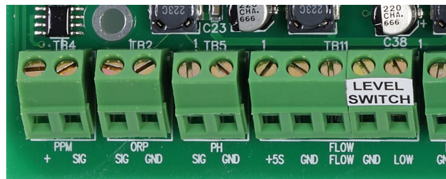
Figure 53. Level Switch inputs (PC 3000 and above)
