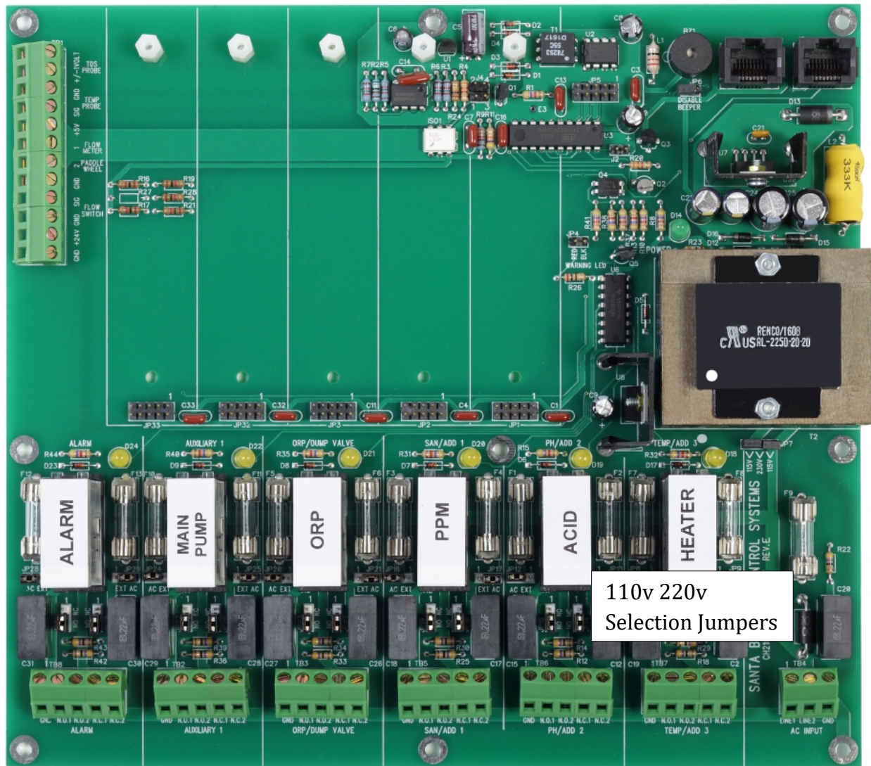
Figure 13. CH2100 Power Supply
