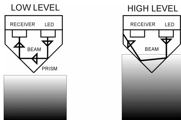
Figure 51. Optical Beam Path
