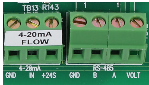
Figure 45. 4-20 mA Flow Meter Connections to PC 3000, PC 5000, pc 5100, PC6000, pc7000and PC 7100
