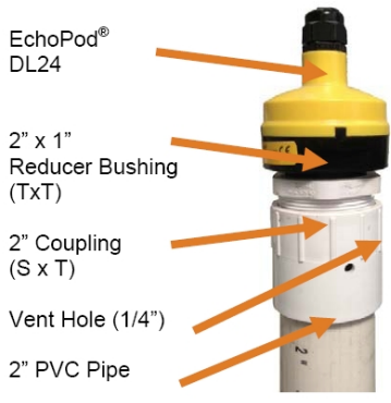
DL24 attached to a LM52-1400 (2"x1" reducer bushing) and 2" Coupling (S x T).
