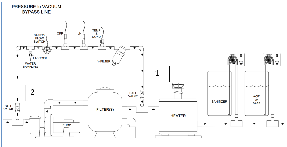
Figure 6. Pressure to Vacuum Bypass Line
