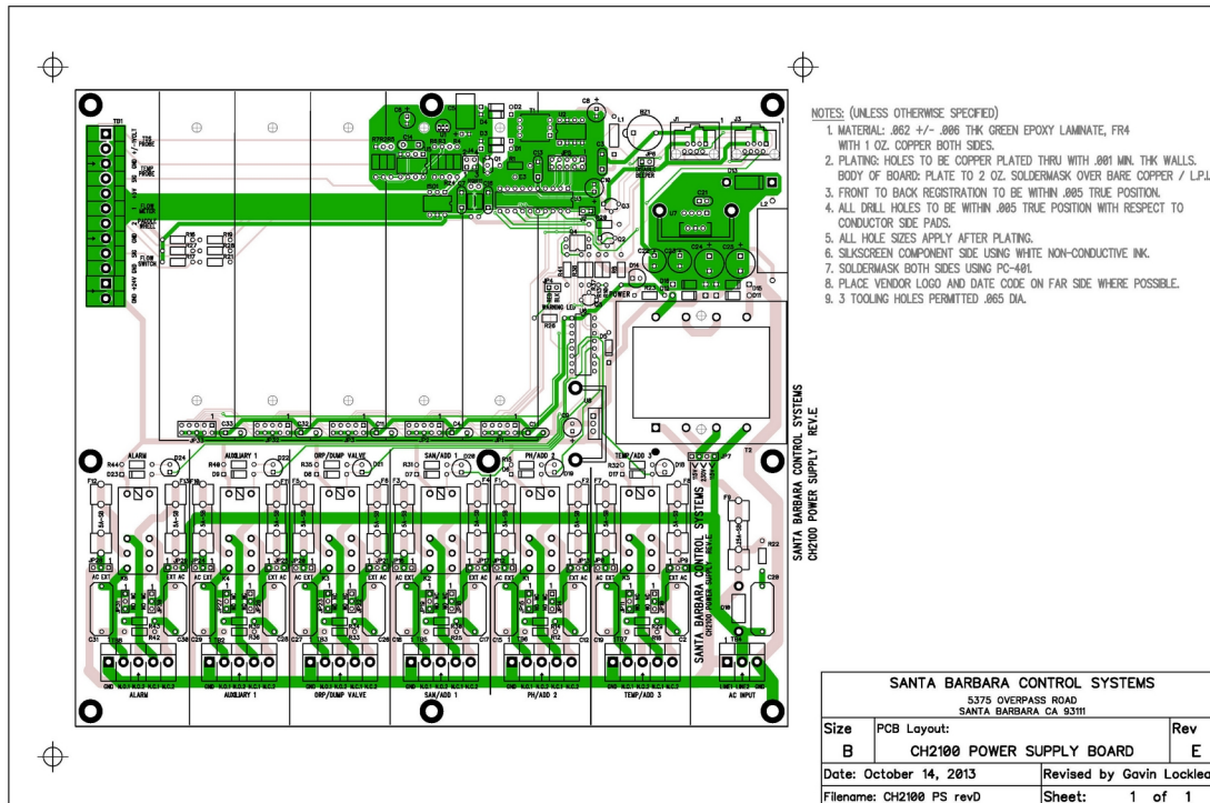
Figure 14. CH2100 Power Board
