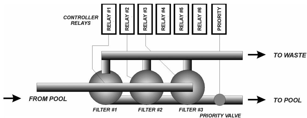
Figure 56. Multiple Filter Backwash
