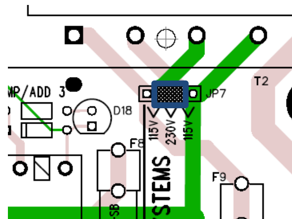
Figure 16. Voltage Selector Jumper set to 230 volts (1 jumper in center) 110v both (2) jumpers cover 4-pins
