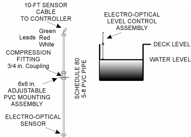
Figure 52. Water Level Assembly
