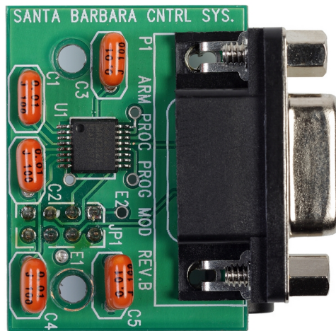
Figure 25. RS-232 Adapter
