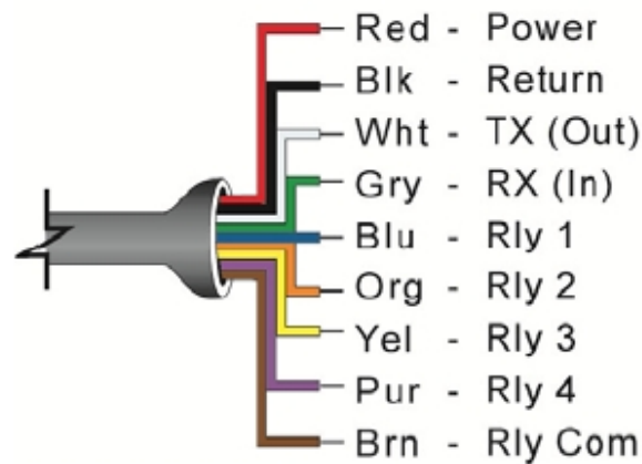
Figure 49. DL24 Wiring
