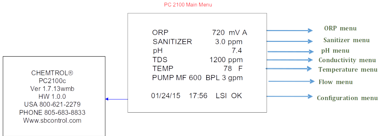
Figure 60. Typical Main Menu for PC 2100 series controllers
