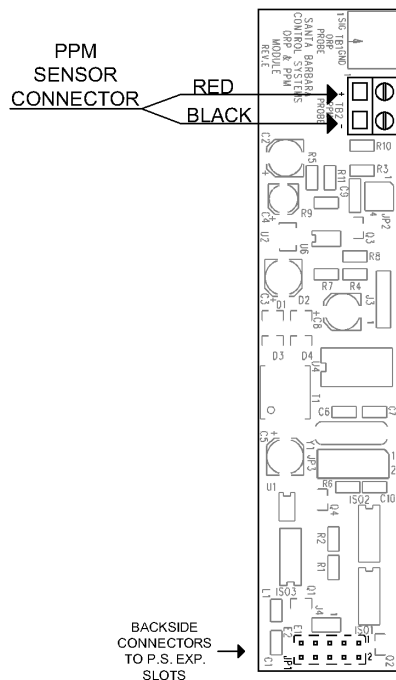
PC1555 PPM SENSOR MODULE
